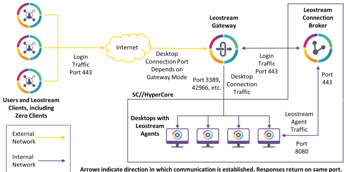
Leostream Remote Access Network Architecture
